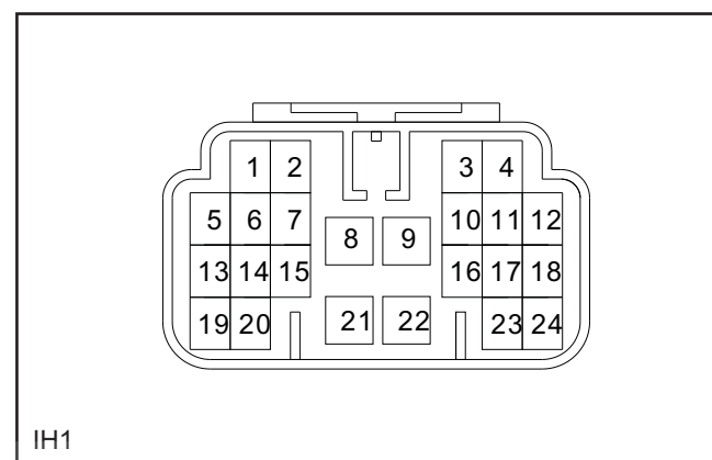
I/P harness to Door harness(LF) Connector
