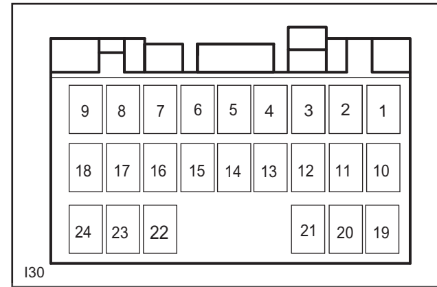
I30 Pin Definition
