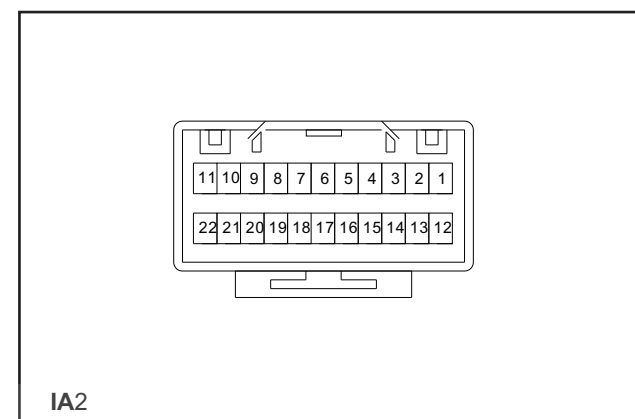
IA2 Pin Definition
