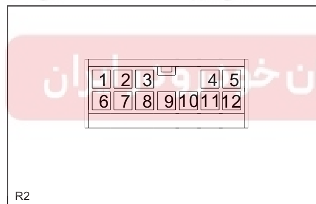
R2 Pin Definition
