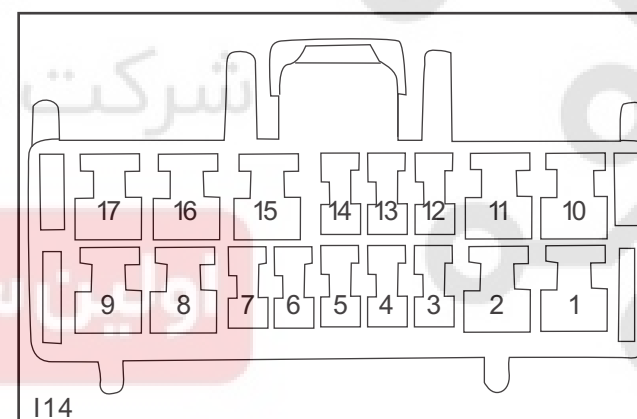
I14 Pin Definition
