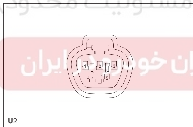
Front Wiper Motor Connector
