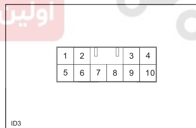
I/P harness to Body harness connector
