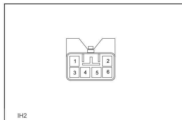
IH2 Pin Definition
