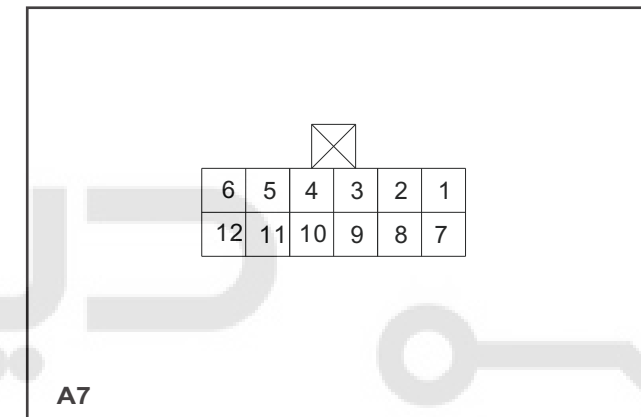
HAVC Connector
