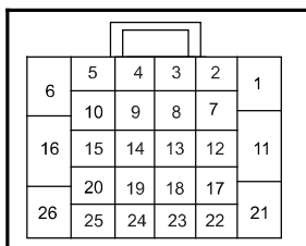
I1_RPAB Reversing Radar W.H.Connector 2 Connecting Body W.H.
