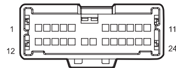
I2_MB Main W.H. Connector 2 Connecting Body W.H.
