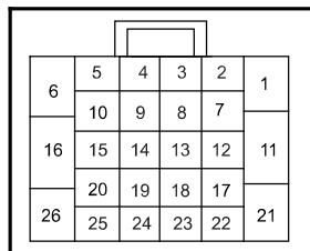
I1_RPAB Reversing Radar W.H.Connector 1 Connecting Body W.H.
