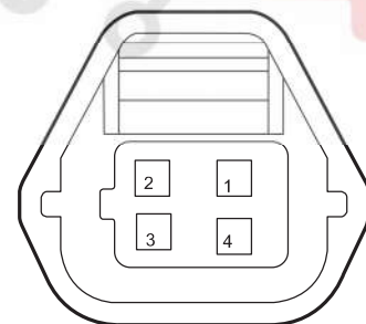
P09 RL Radar(low-line)
