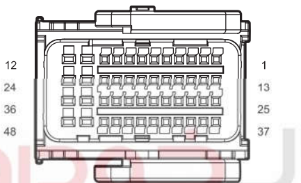
F01 BCM C2
