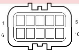
I_FB-ENG Front Bumper W.H. Connector Connecting Engine Compartment W.H.
