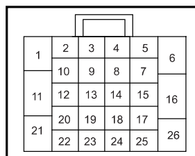
I1_BRPA Body W.H. Connector 2 Connecting Reversing Radar W.H.
