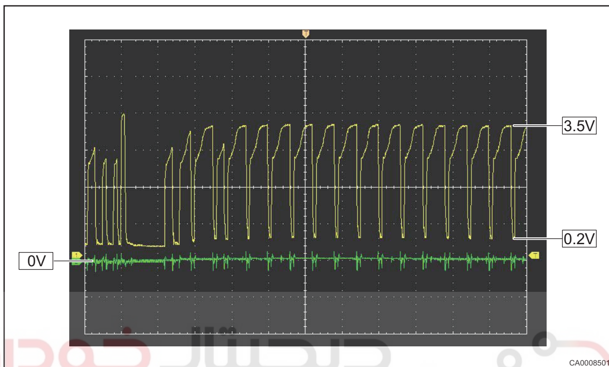
Power CAN malfunction waveform
