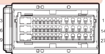
I2_MF Main Harness to Body
