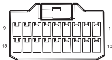
I1_MR Main Harness to Roof Harness
