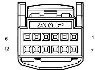
R13 Front Roof Lamp(Top-line)
