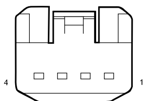
R08 RL Roof Lamp
