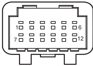
D07 Left Rear View Mirror
