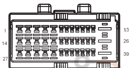
I1_FM Body Harness to Main Harness I
