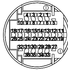
E44 DCT Transmission
