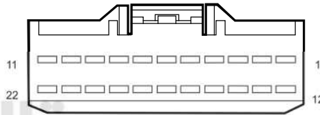
I4_ME Main W.H. Connector 4 Connecting Engine W.H.
