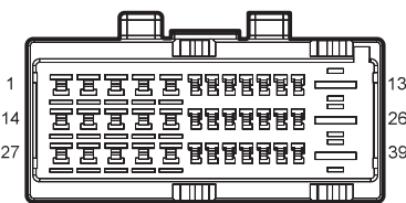
I2_FM Body Harness to Main Harness I1
