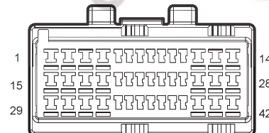
I1_EM Engine Harness to Main Harness 1
