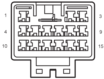
I3_FD Body Harness to Left Rear Door Harness
