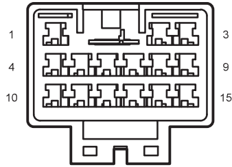
I4_FD Body Harness to Right Rear Door Harness
