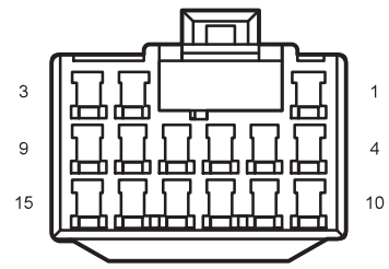
I4_DF Right Rear Door Harness to Body Harness
