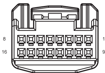
D05 Left Front Door Main Switch(High Spec)
