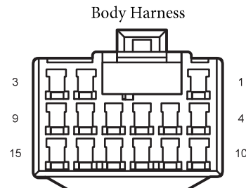
I4_DF Right Rear Door Harness to Body Harness
