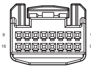
D05 Left Front Door Main Switch(High Spec)
